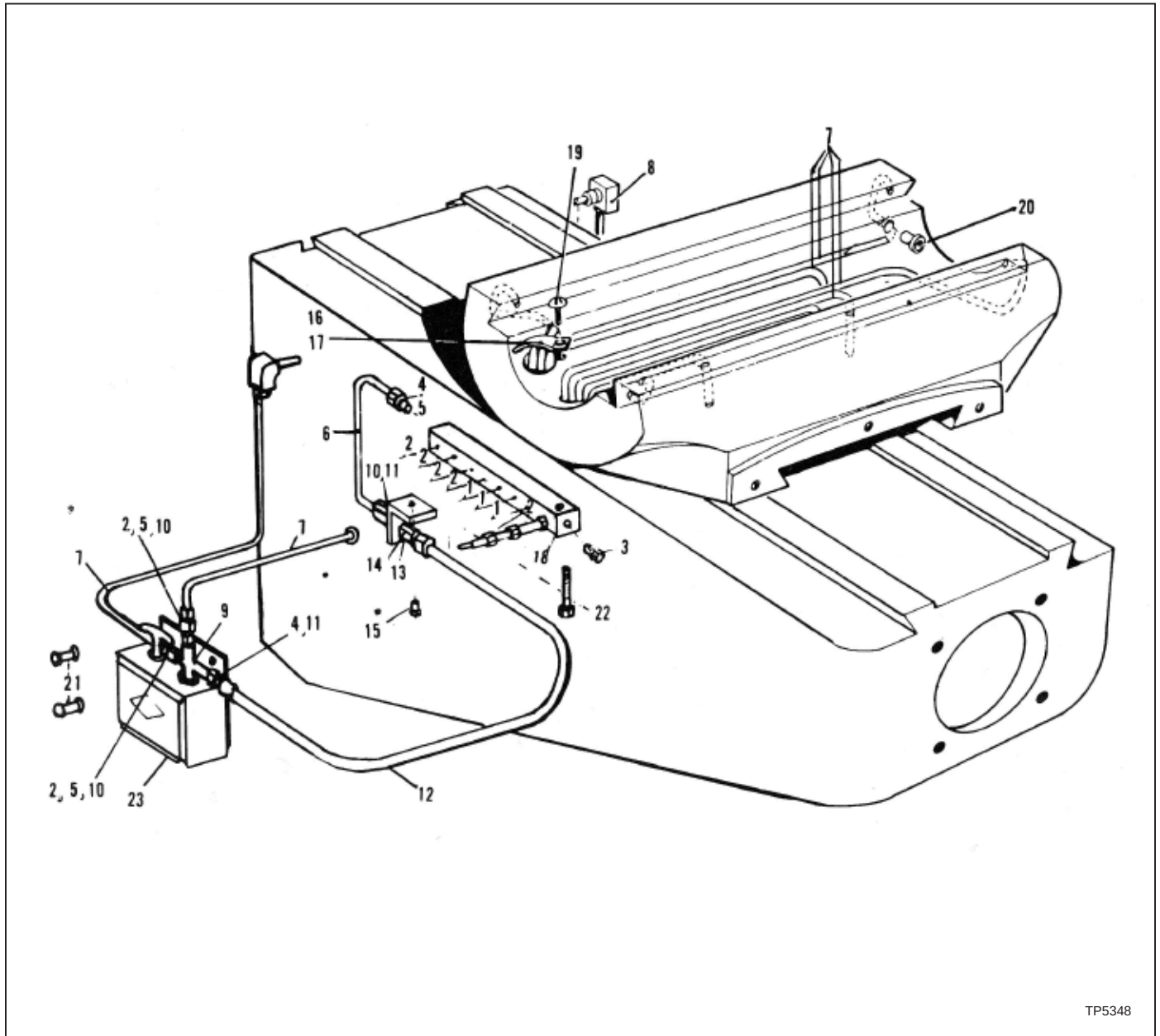
Figure 4.10 - Lubrication System Assembly
