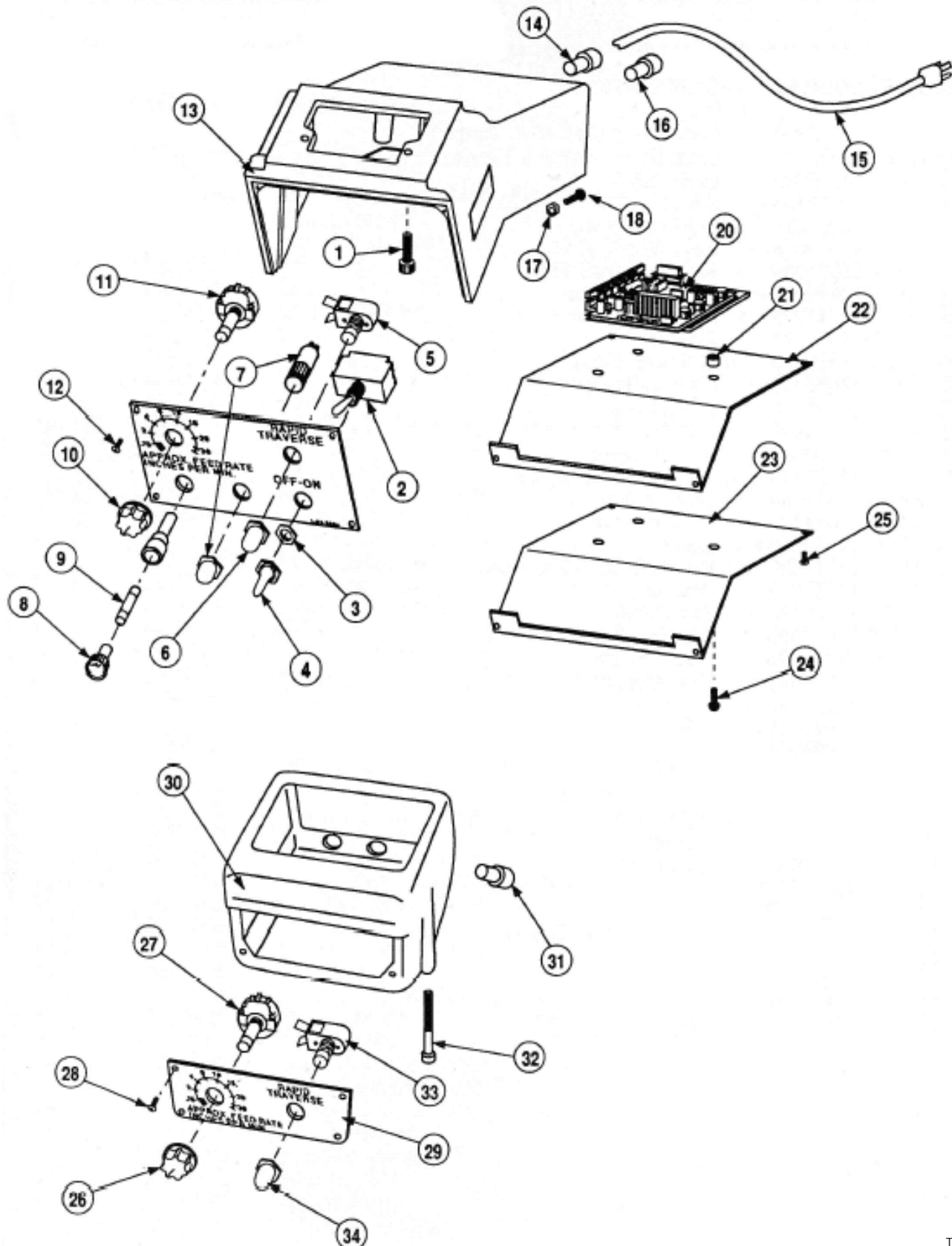
Figure 4.17 - 8F Power Feed X-Axis Control Assembly, Exploded View
